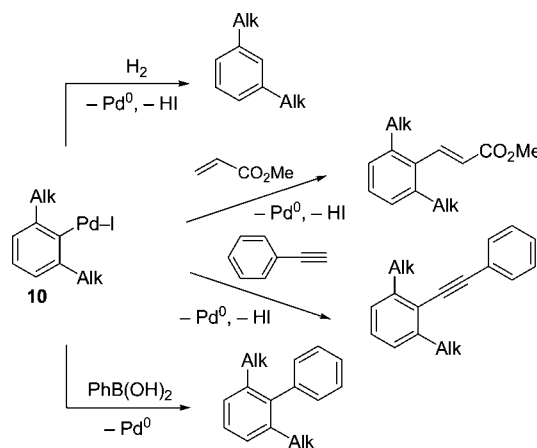
SCHEME 3. Termination Steps
