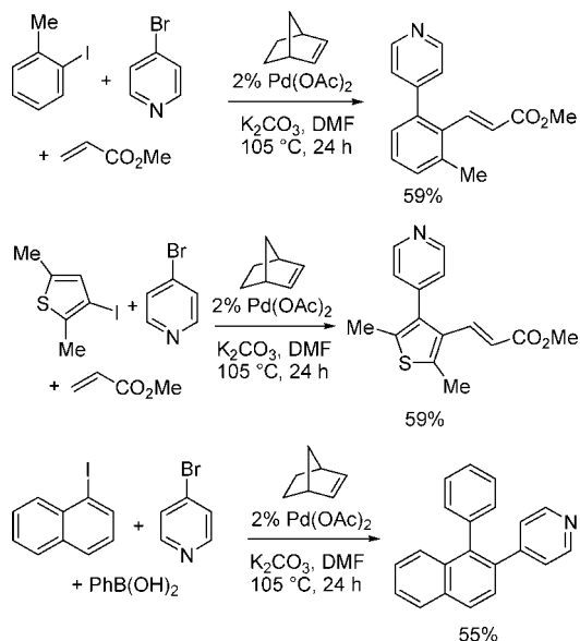
SCHEME 12. Heteroatom-Containing Coupling Products
