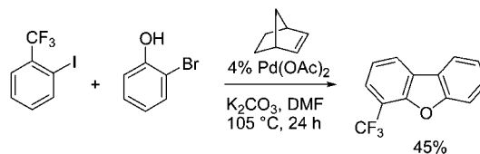
SCHEME 14. 4-Trifluoromethyldibenzofuran
