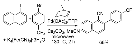
SCHEME 11. 2-(4-Trifluoromethylphenyl)-1-naphtho-nitrile
